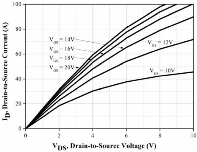
Figure 3. Output Characteristics T_j = 150^\circ\text{C}
