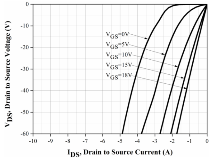
Figure 10. 3 rd quadrant characteristic at T_j = 25^\circ\text{C}
